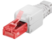
MicroConnect Cat 6 Tooless RJ45 Plug MPN: KON520TL
